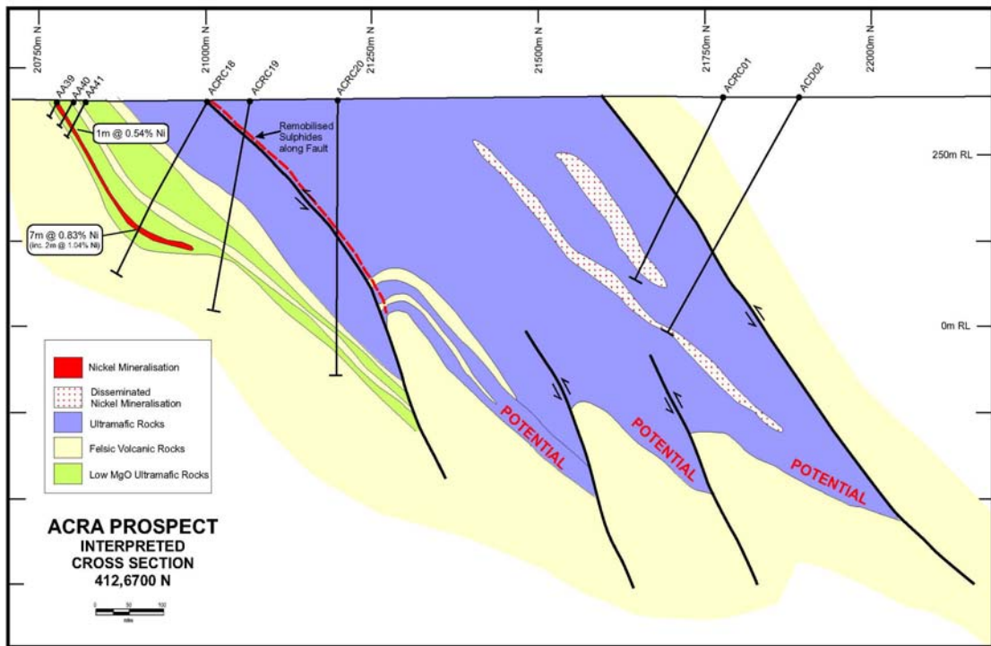
Figure 2: Schematic Cross Section of the Acra Prospect
